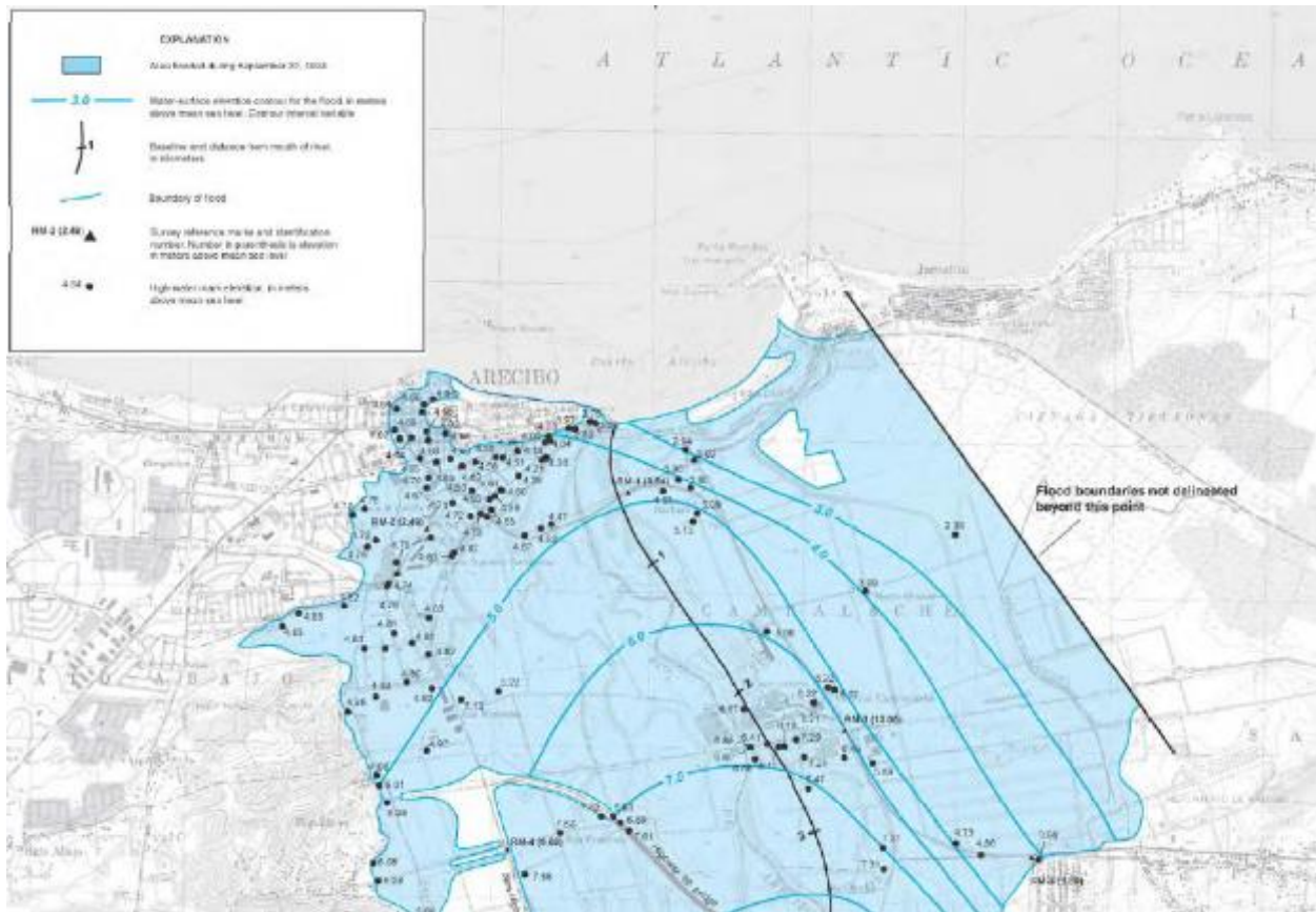
Figure 3-8. Area Inundated as a Result of Hurricane Georges
