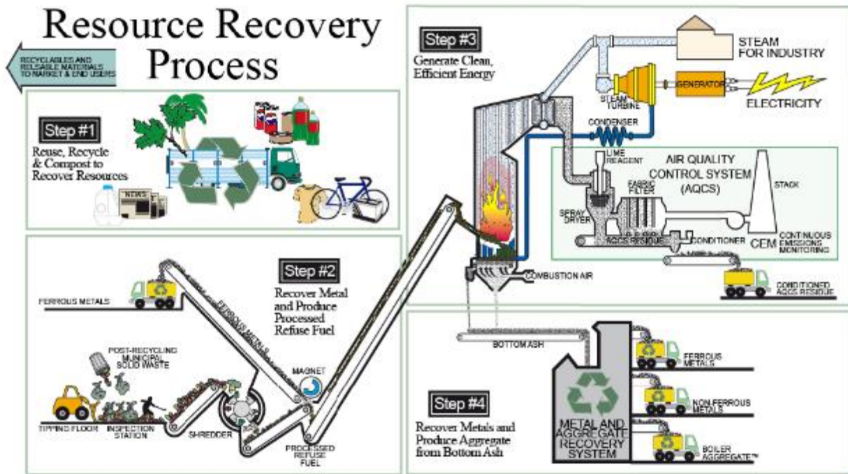
Figure 2-4. Simplified Power Generation and Resource Recovery Process Flow Chart
