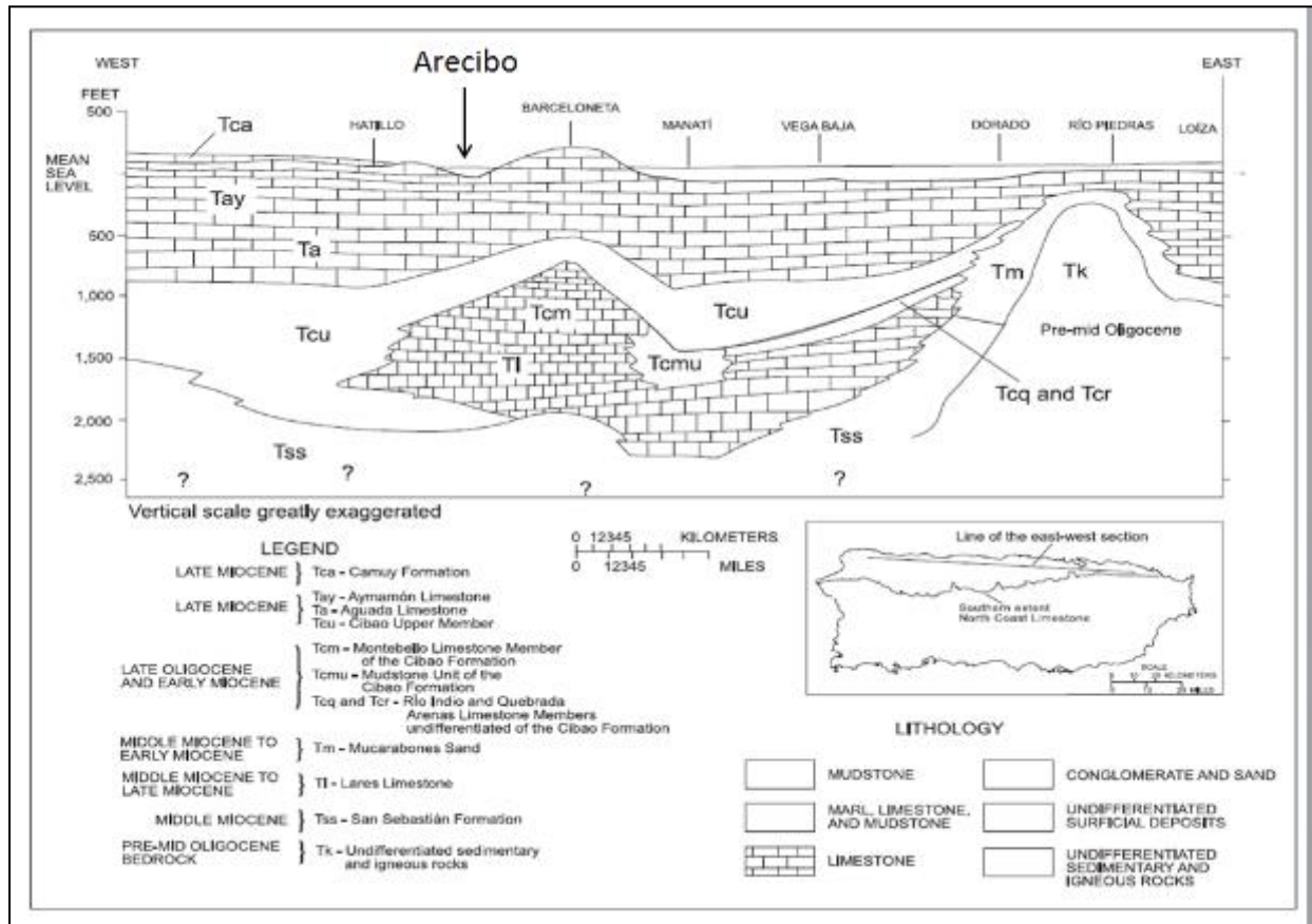
Figure 3-1. Regional Geologic Section of the Northern Karst Belt
