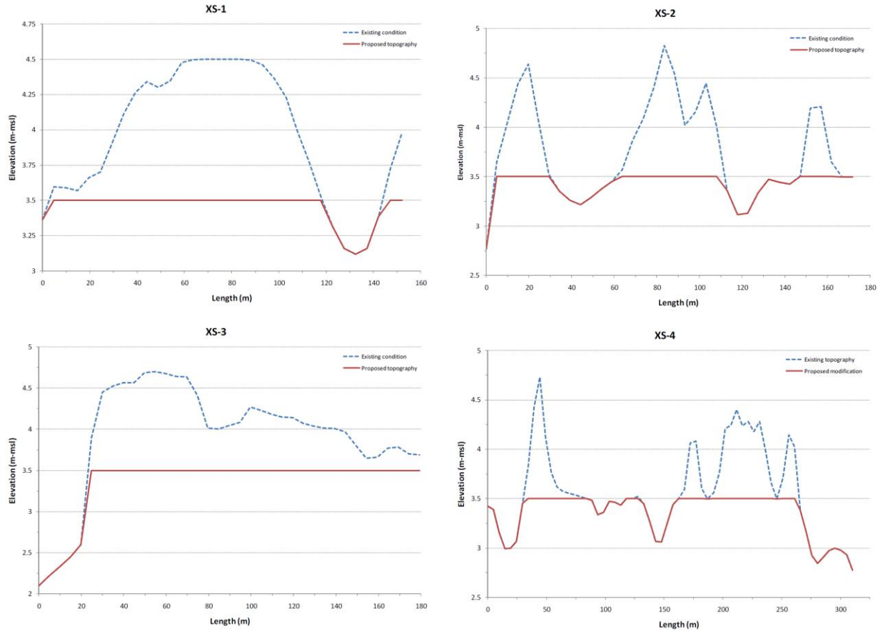
Figure 3-9. Proposed Geometry of Bank Modification Area
