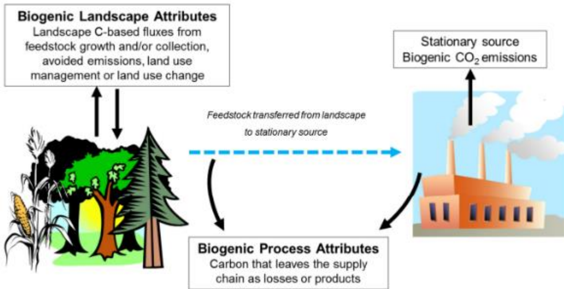
Figure 3-11. Conceptual Illustration of Carbon Fluxes between Landscape/natural Systems and Stationary Sources
