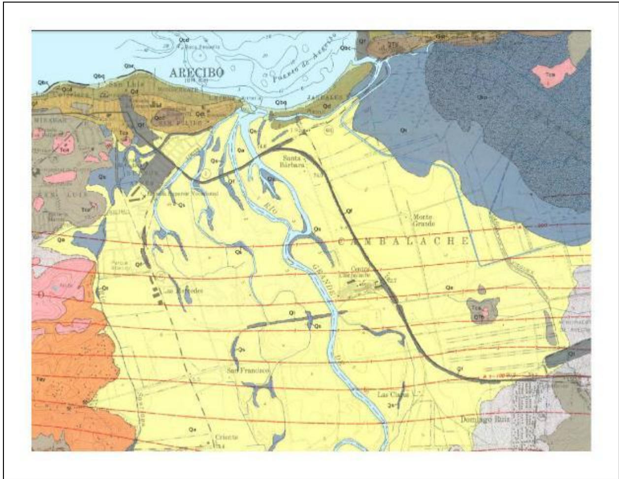
Figure 3-2. Regional Geologic Map
