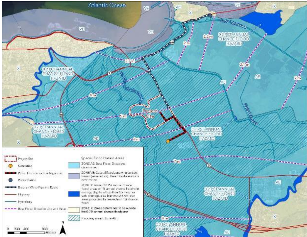
Source: FEMA (2015), NRCS (2014), digitized by Louis Berger Figure 3-5. FEMA Flood Insurance Rate Map, Panel 230J
