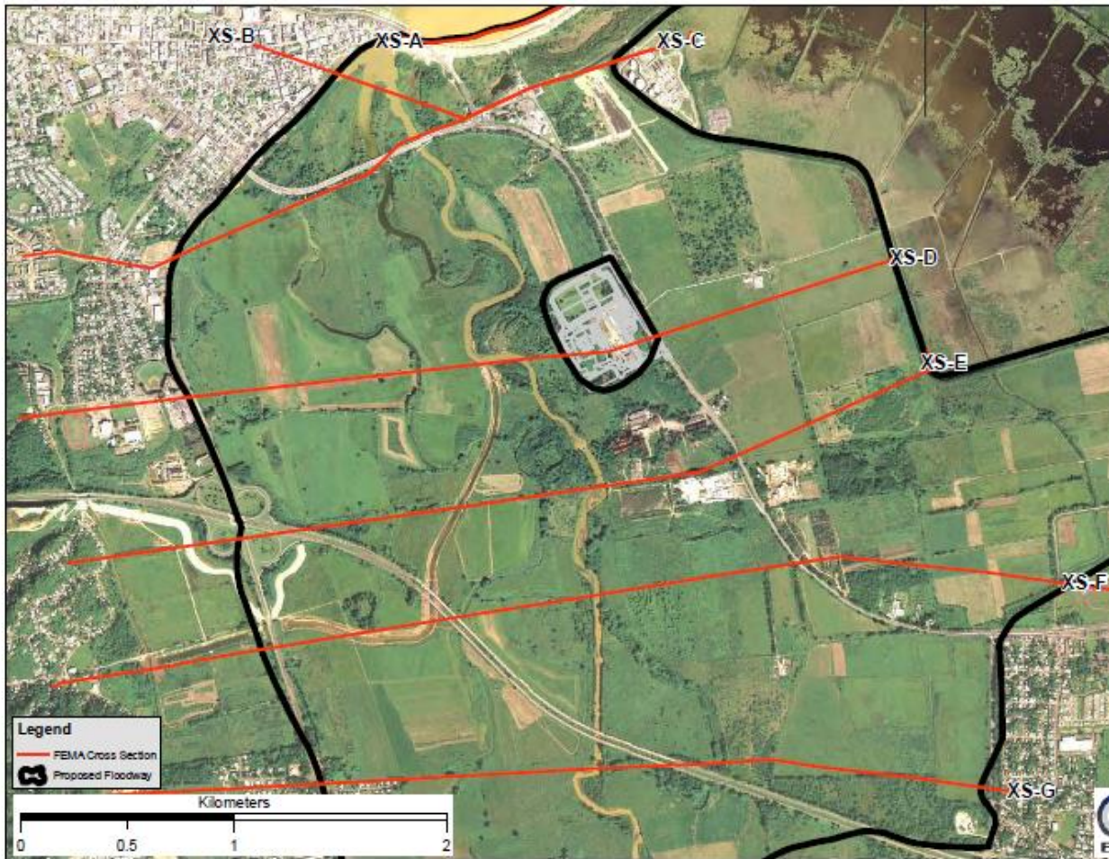
Figure 3-6. Proposed 100-year Floodway Limit and Cross Sections
